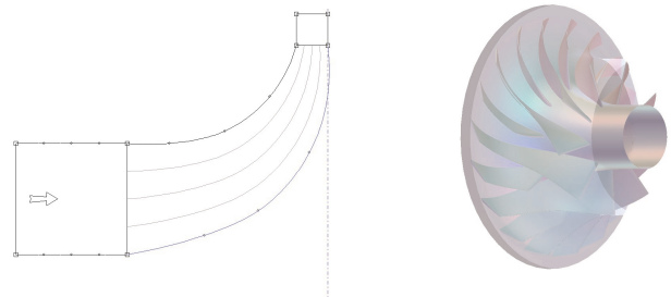
Fig. 3 Instantly-launched 3D geometry in BladeModeler™.
