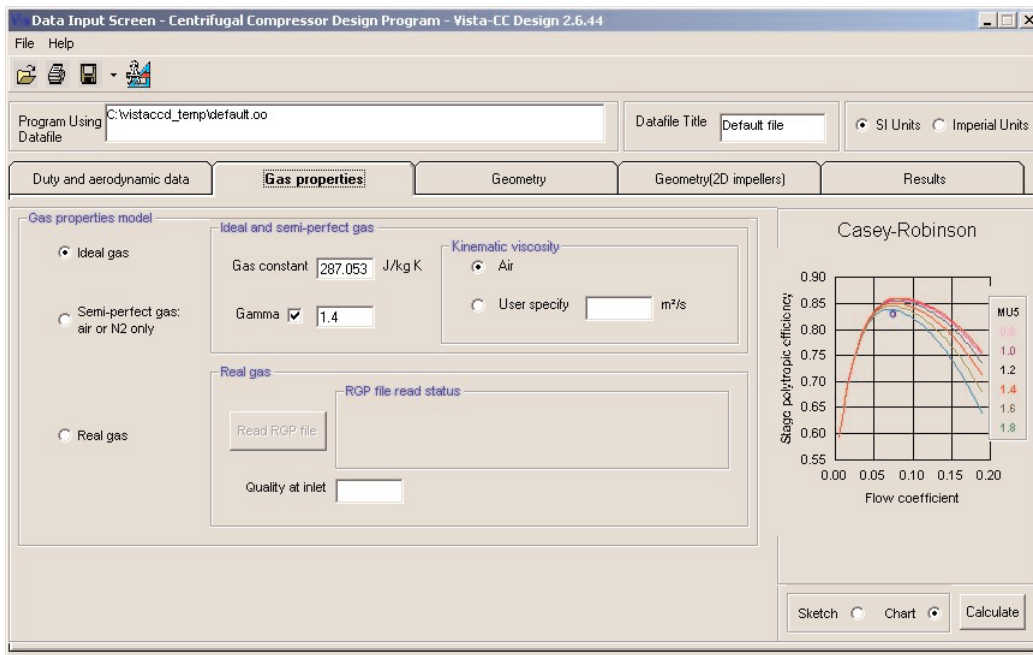
Fig. 2 Vista CCD user interface
